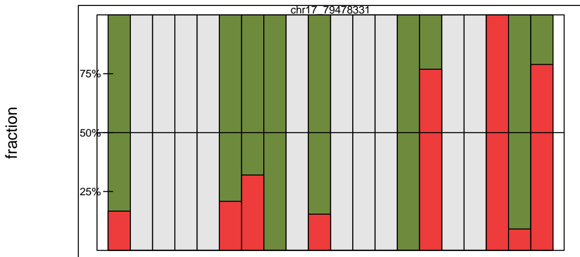
Figure 7: A barplot with the maternal phase as top fraction, top.fraction.criteria='phase'
