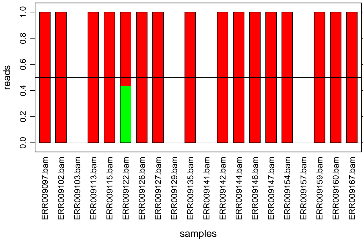
Figure 11: A gbarplot with type='fraction'
