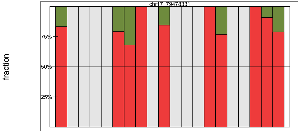
Figure 6: A barplot with the reference allele as top fraction, top.fraction.criteria='ref'
