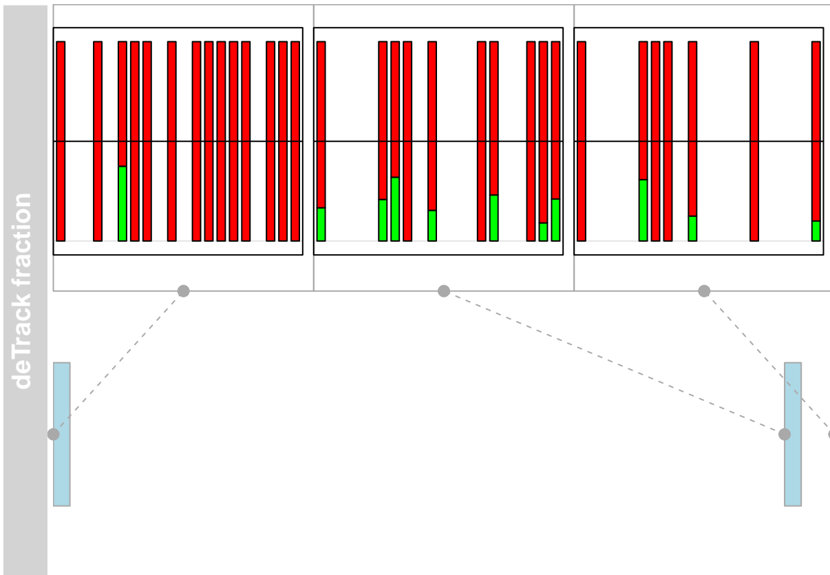
Figure 12: A glocationplot, showing the ASE of SNPs within a defined region
