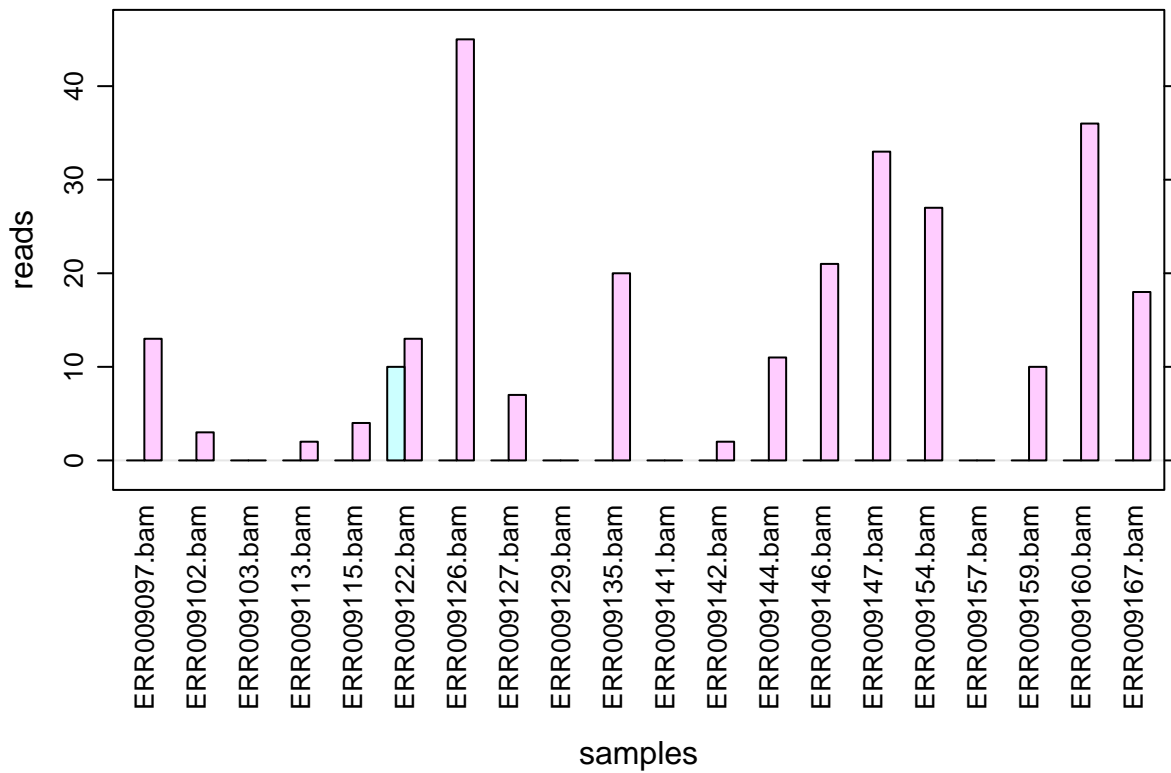
Figure 10: A gbarplot with type='count'
