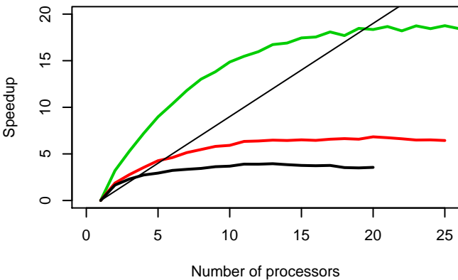
Invariantset Normalization
