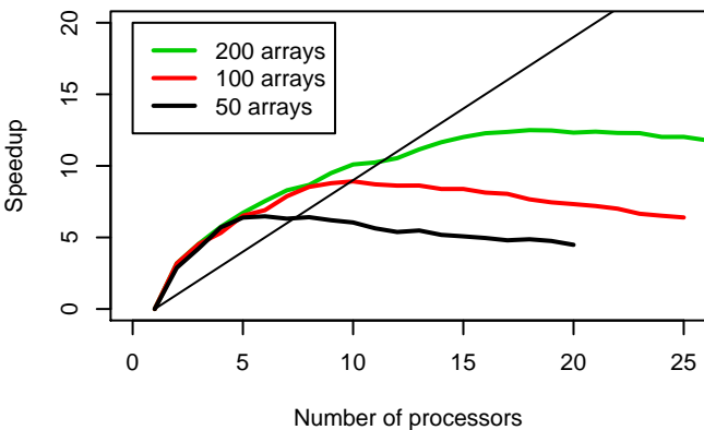
Constant Normalization
