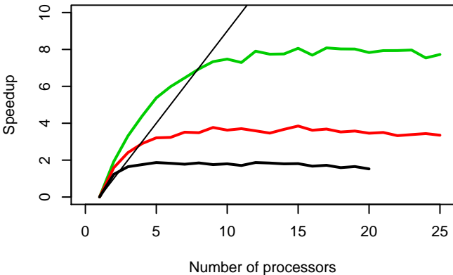
Invariantset Normalization
