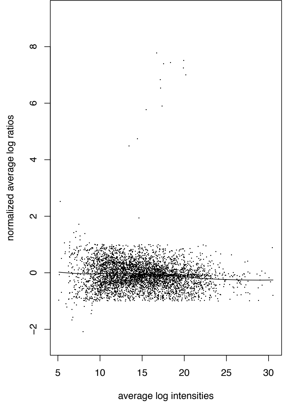
Normalized average log ratios versus average log intensities
