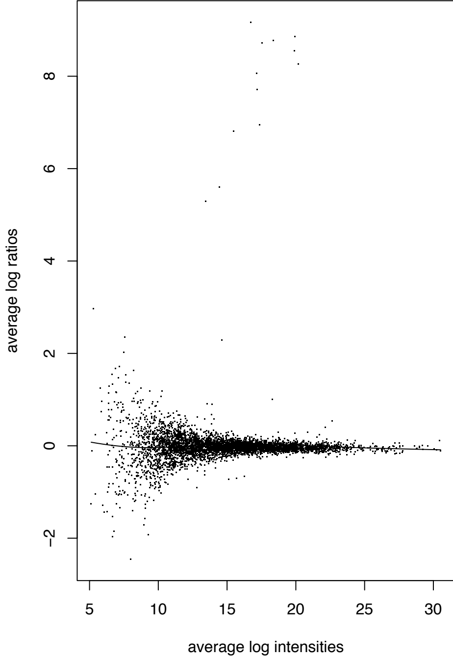
Average log ratios versus average log intensities
