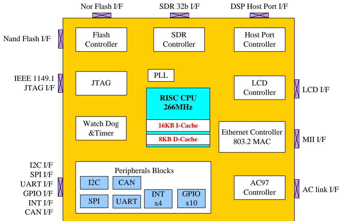
SOC3210M Function Block Diagram
