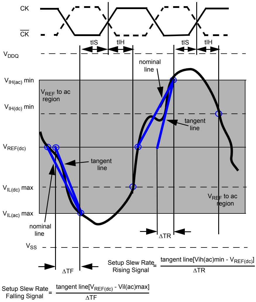
Figure 14 - Illustration of tangent line for t1S
